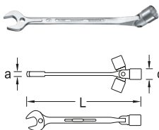
534 Combination swivel head wrench
